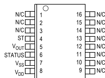
Figure 2. Pin Connections
